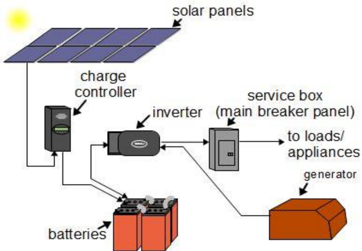
Solar panel off grid system
