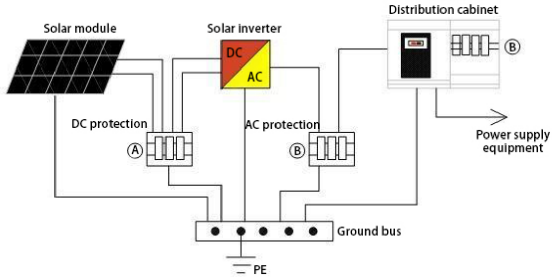
Schematic Diagram of the Inverter in Solar On Grid Power System
