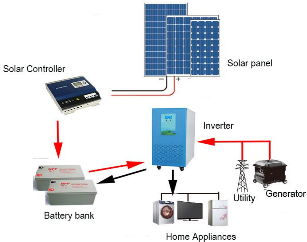
Inverter off grid system
